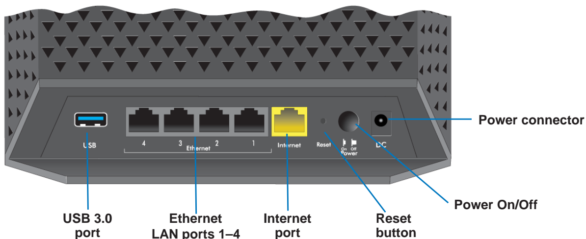
Figure 3. Router rear panel
